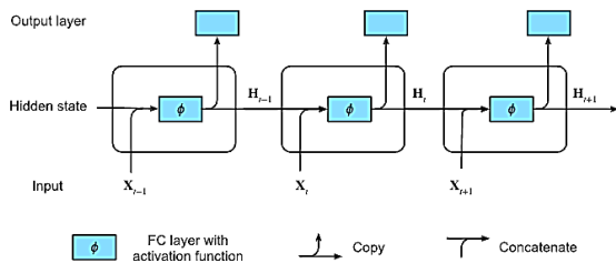
Figure 6: Basic illustration of RNN
