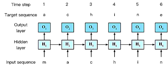
Figure 7: RNN-based Character-Level Language Models
