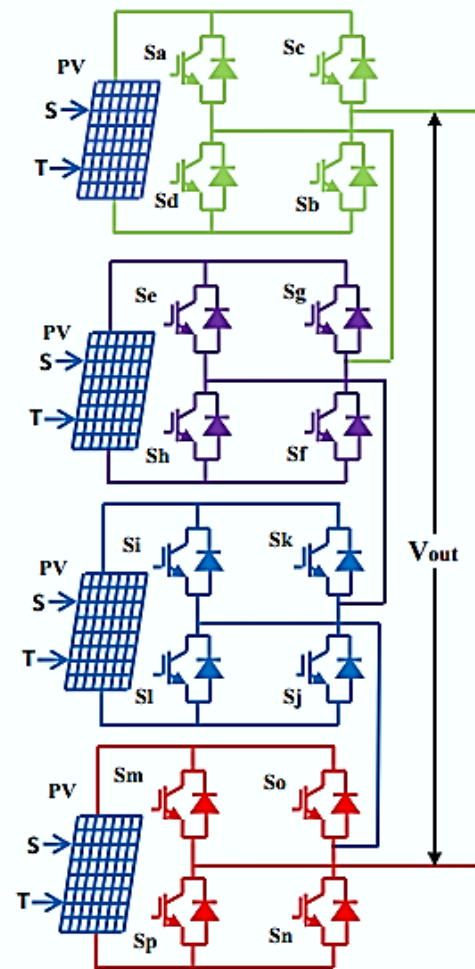
Figure 4: Circuit diagram of 9-level CHBMLI
