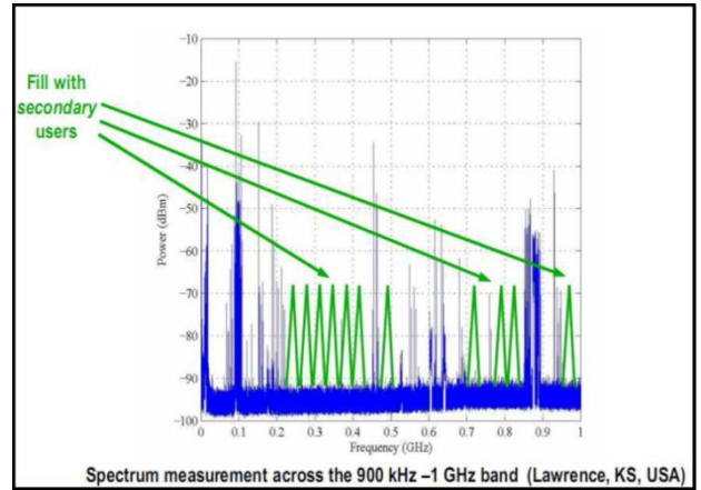
Figure-2: Spectrum Measurement across the 900 kHz-1 GHz (Lawrence, KS, USA) (a) Frequency holes (b) Fill those holes with secondary user’s data
