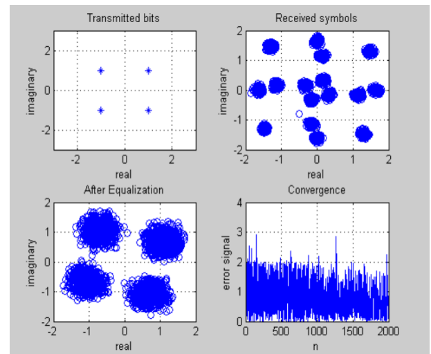
Fig. 5 Performance through Blind equalization
