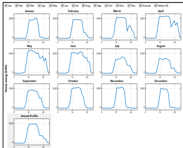
Fig 4.10- Every Month Energy
