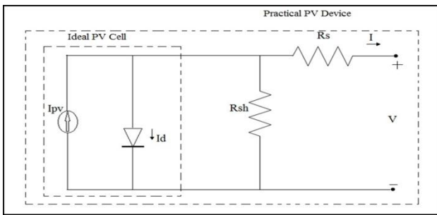
Fig-3.1: Equivalent circuit of a practical PV device [6]
