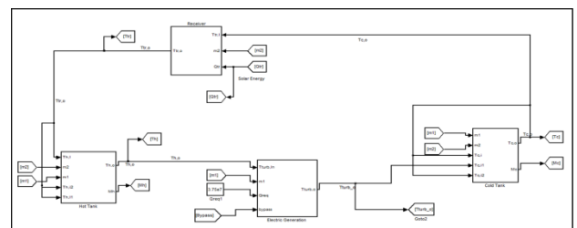
Fig 4.1- Simulink model of the CSP plant with storage system
