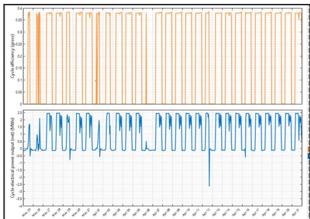
Fig 4.8-Cycle Efficiency and Net Electrical power output
