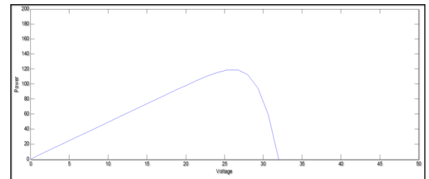
Fig 3.4-P-V Characteristic
