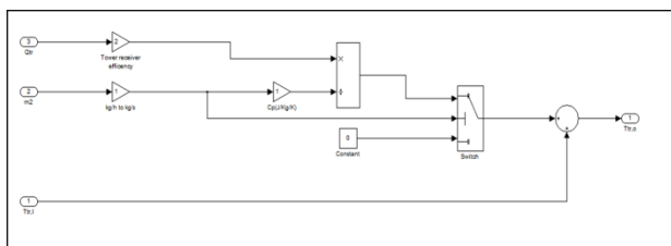
Fig 4.2 Receiver subsystem for outlet temperature modelling
