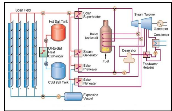
Fig 1.2-Components of CSP with TES (Thermal Energy Storage)
