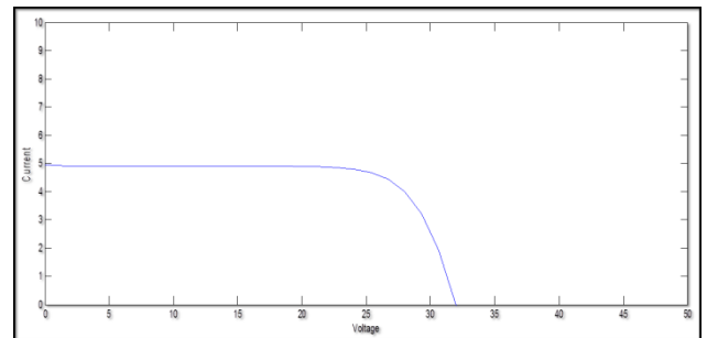
Fig 3.3-I-V Characteristic
