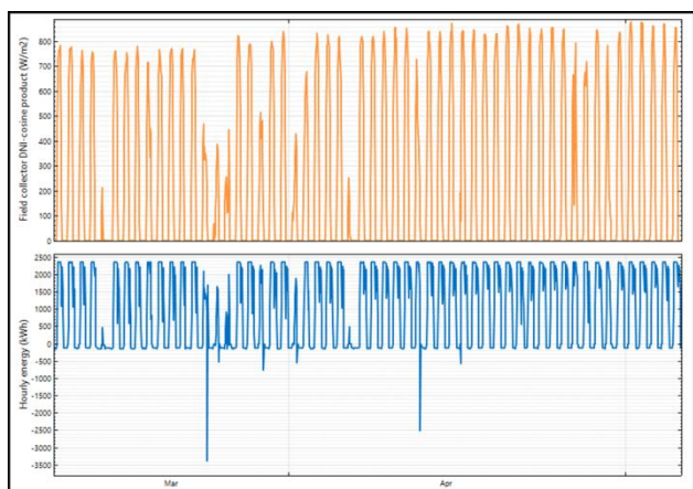
Fig 4.9-DNI and Hourly Energy
