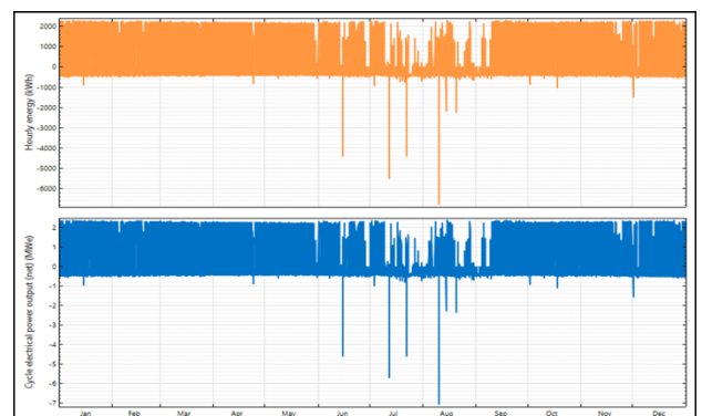
Fig 4.6- Hourly energy and Inlet & cycle net electrical power
