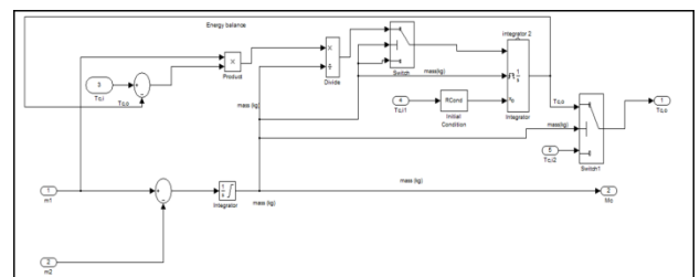
Fig 4.5-Cold tank subsystem designed with Simulink
