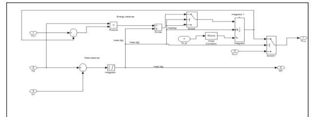
Fig 4.3- Hot tank subsystem designed with Simulink
