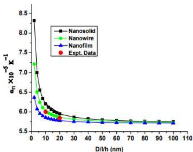
Fig. 4 Volume thermal expansion coefficient \alpha_V as the function of cluster size D of Ag nanomaterial. The solid lines with symbol represent the model prediction. are used for calculation for Ag nanosolid, nanowire and nanofilm respectively. The symbol \bullet shows the experimental results of Ag nanowire
