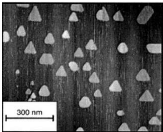
Figure 3: Morphology of prism shaped indium in nanoparticles
