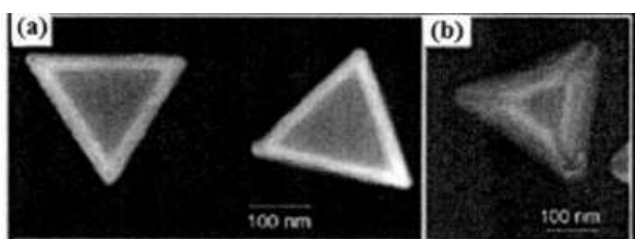
Figure 2: Different morphologies of Au nanoparticles like (a) truncated tetrahedral and (b) tetrahedron
