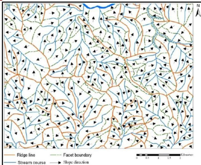
Figure 3 Slope facet of Mussoorie
