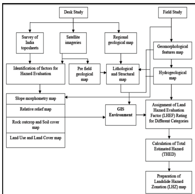
Figure 1 Flow chart showing the process followed for landslide hazard macro zonation mapping.
