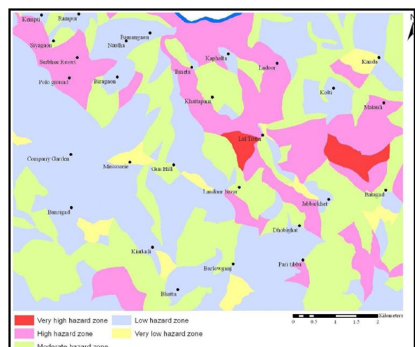
Figure 1 Landslide hazard zonation map
