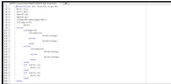
Fig 9- MPPT Algorithm of Solar PV System
