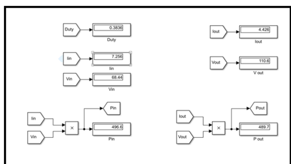
Fig 12- Solar PV array Observation Table
