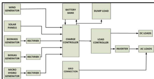
Figure 4 Basic Diagram of Hybrid System
