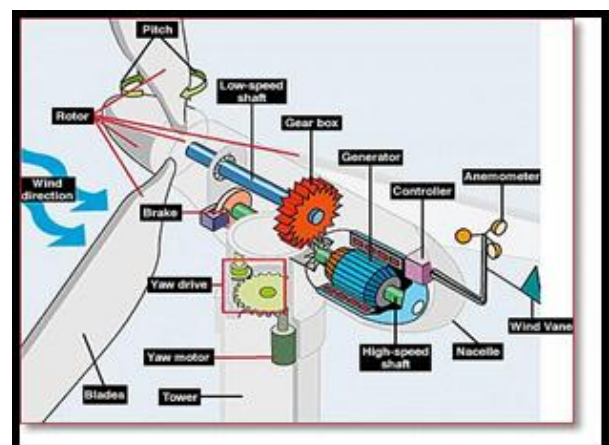
Figure 3 The Main component of a Wind Turbine can be classified as i) Tower ii) Rotor System iii) Generator iv) Yaw v) Control System vi) Breaking and Transmission System hybrid operation and smart grid
