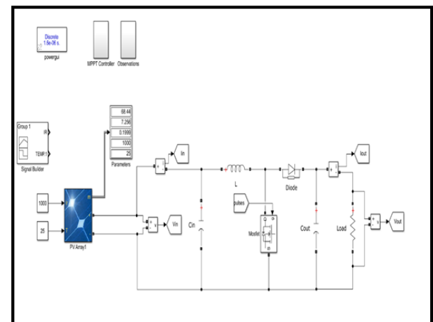
Fig 7- Solar PV Array Simulation with MPPT & Boost Converter
