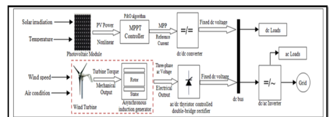
Figure 6 Block diagram of the proposed system
