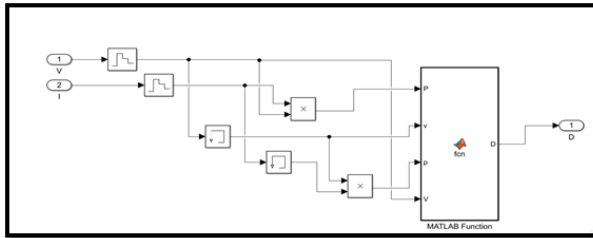
Fig 8- MPPT Subsystem of for the Solar PV
