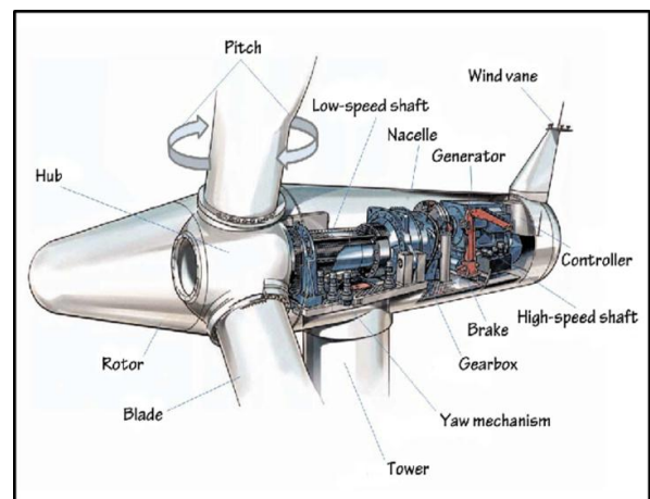
Figure 2 Major Component of Wind Turbine
