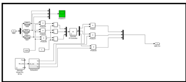
Fig 20 PI Controller Subsystem
