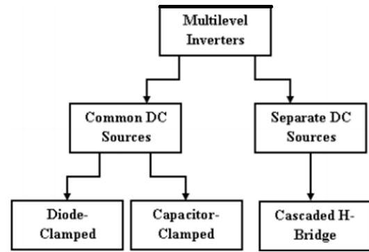
Figure 1: Multilevel Inverter Topologies
