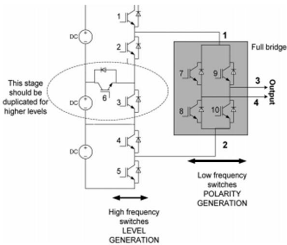
Figure 2: Schematic of a seven-level inverter in single phase
