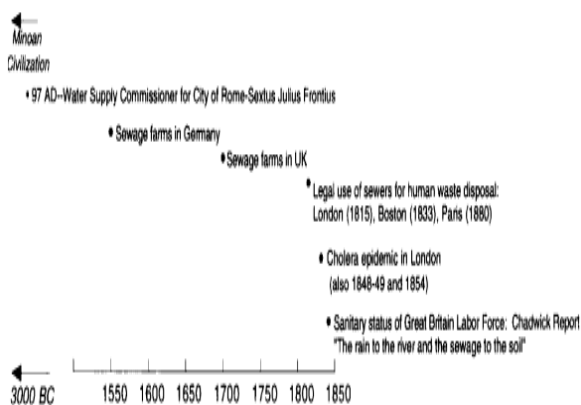
Figure 2: Early systems of water and sanitation
