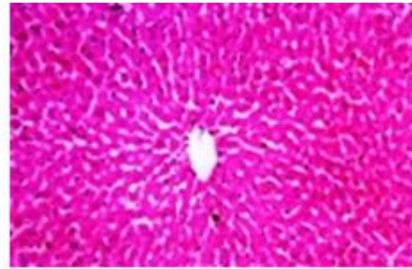
Figure 9: TS of normal liver (Group-I).
