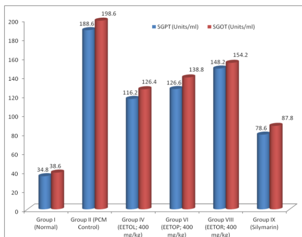
Figure 13: Effects of EETOL, EETOP, EETOR & Silymarin on SGPT & SGOT.
