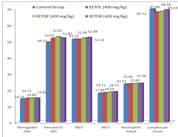
Figure 7: Effects of EETOL, EETOP and EETOR on blood parameters.
