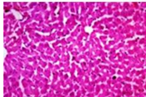
Figure 11: TS of EETOL (400 mg) treated liver
