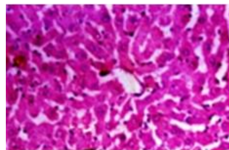
Figure 12: TS of Standard reference drug i.e. Silymarin treated liver.
