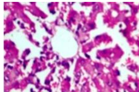
Figure 10: TS of PCM induced toxicity (Group II).
