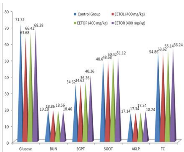
Figure 8: EETOP, EETOL and EETOR effect on LFTs.
