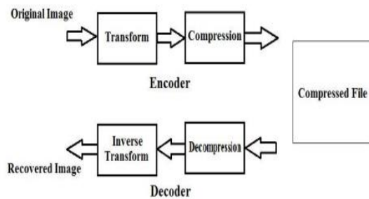
Fig 1: Image compression [7]
