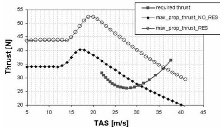
Fig. 7 Propeller thrust versus required thrust
