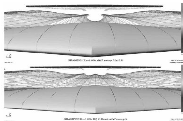
Fig. 9 Downwash blended zone
