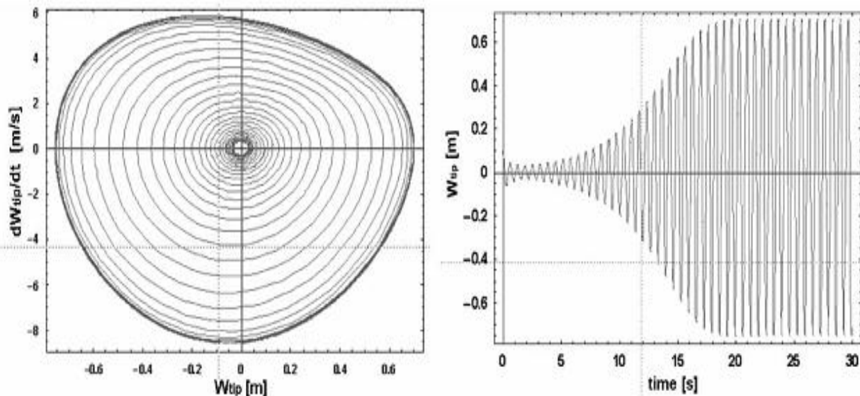
Fig. 17 Limit cycle oscillations (LCO) in the supercritical regime
