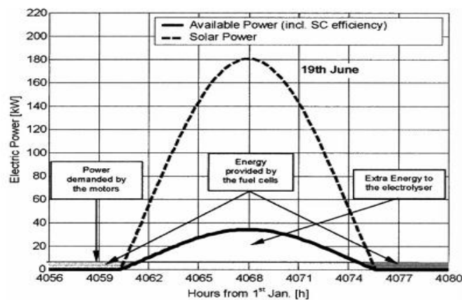
Fig. 4 Solar power distribution and energy balance
