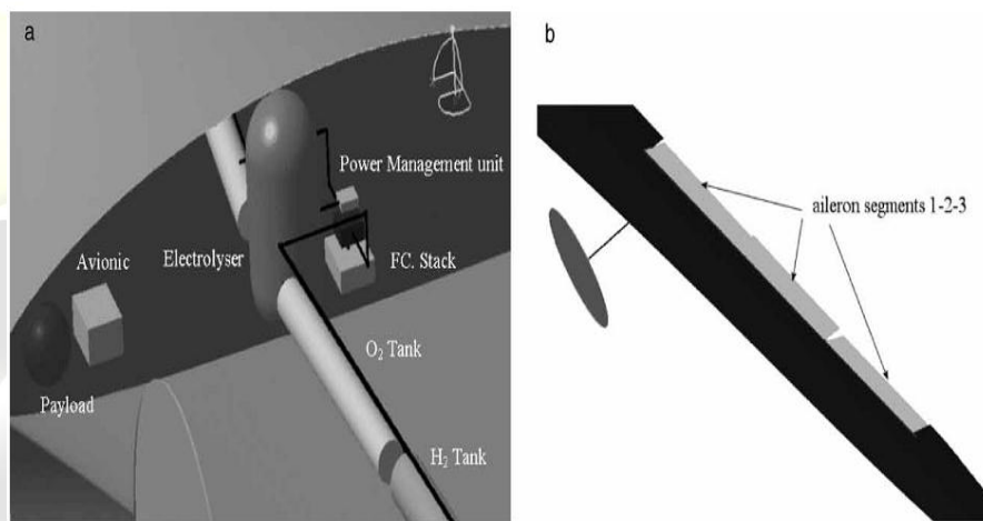
Fig. 6 Aileron segments and internal layout
