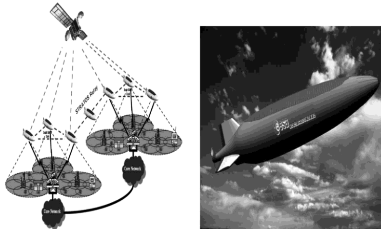
Fig. 3 Aerostatic HAVE-UAV for telecom applications
