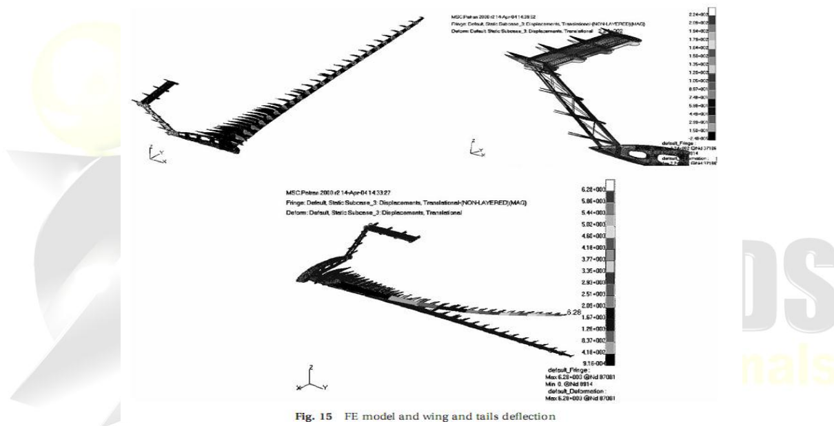
Fig. 15 FE model and wing and tails deflection
