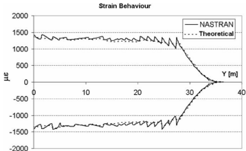
Fig. 14 Strain behaviour along wing span
