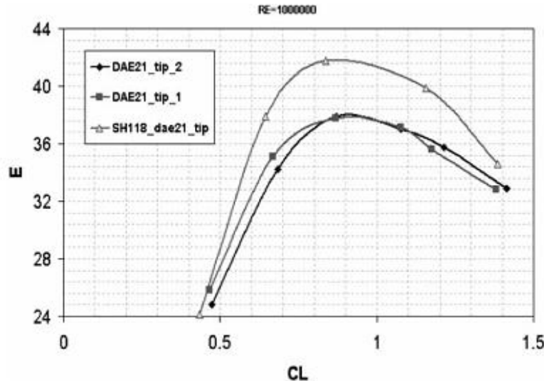
Fig. 10 Aerodynamic efficiency
