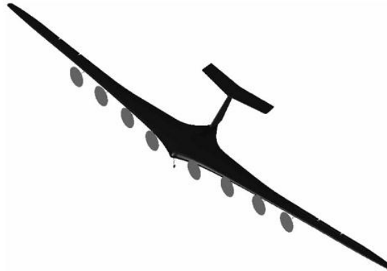
Fig. 8 Shampo configuration, external view
