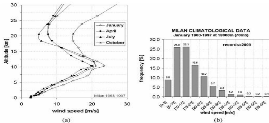
Fig. 5 (a) Average wind speed profile for several altitudes and seasons. (b) Statistic distribution at 18 km in January
