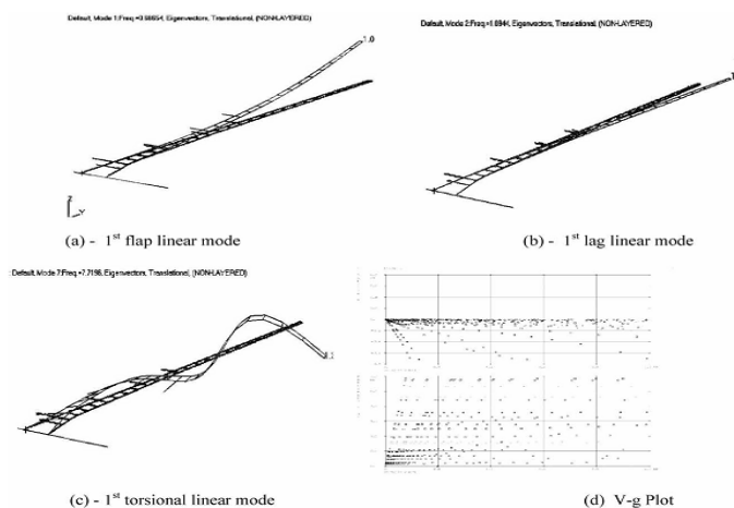
Fig. 16 Linear natural modes and flutter identification
