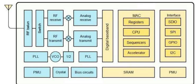
Figure 1: Block Diagram of WSNs.
