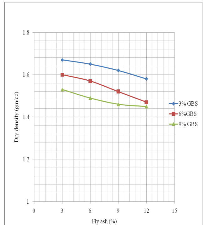
Fig -3: Variation of MDD with fly ash and GBS mix
