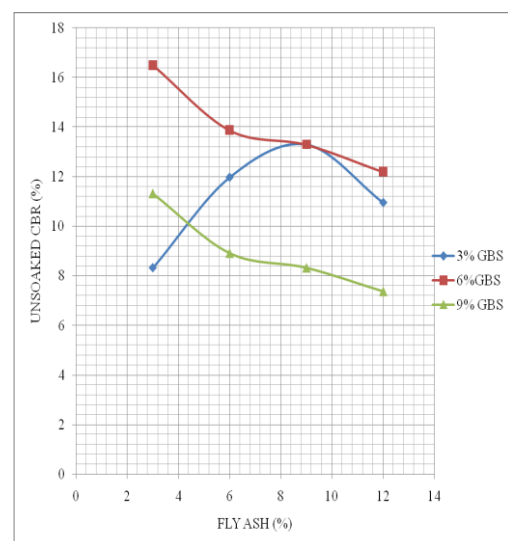
Fig -6: Variation of unsoaked CBR with fly ash and GBS mix
