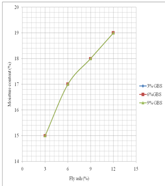
Fig -4: Variation of OMC with fly ash and GBS mix
