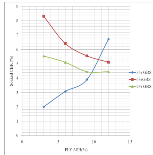
Fig -5: Variation of soaked CBR with fly ash and GBS mix
