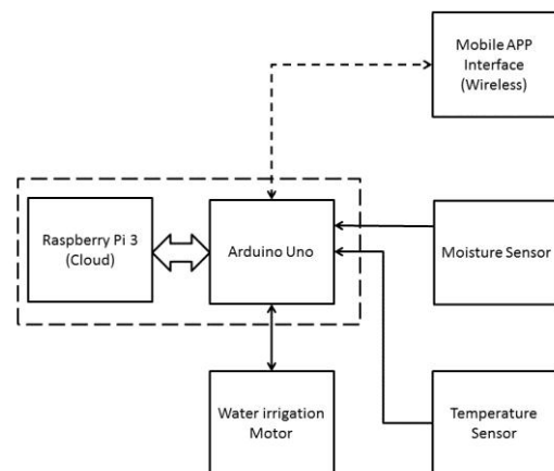
Fig. 6: Block diagram of system
