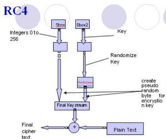
Fig 1: RC4 Algorithm
