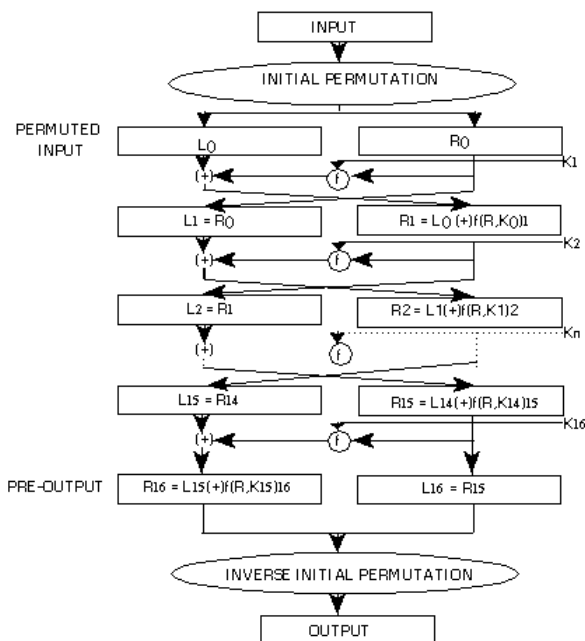
Fig 4: DES Algorithm
