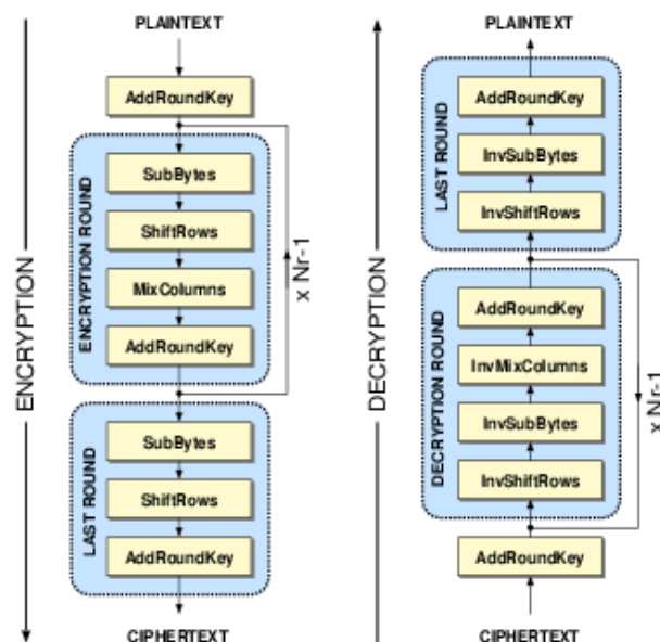
Fig 2: AES
