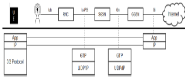
Fig. 2 Structure of 3G Protocol Stack
