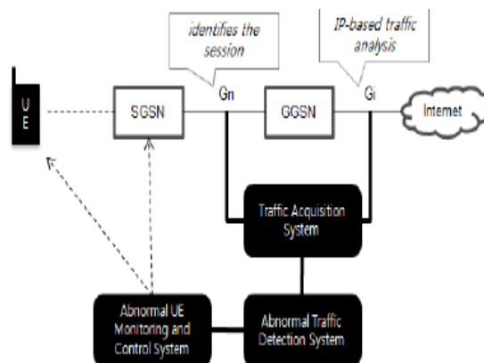
Fig. 4 Framework for optimal security system for the 3G mobile Networks
