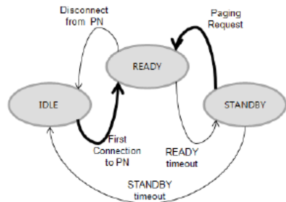
Fig. 3 UE State on 3G mobile network
