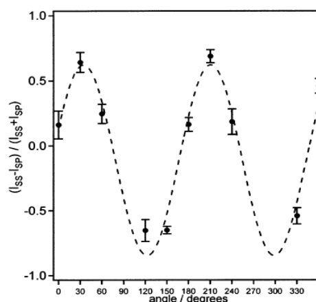
Figure 2. Angle dependence of the polarization parameter F for a representative SERS-active aggregate. The data are collected under the same conditions described in Figure 1. Ten integrations are taken at each angle, with 30^\circ increments. A polarization parameter equal to 1 indicates that the scattering is completely polarized and -1 indicates that it is completely depolarized. The error bars represent \pm 1\sigma_F .
