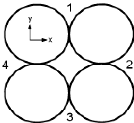
Figure 3. Schematic representation of the difference between Rayleigh and Raman scattering from SERS-active aggregates. The Rayleigh scattering is delocalized over the whole aggregate, which, in this example, is isotropic due to the 4-fold axis of symmetry. (Formally, an axis of symmetry of order three or higher ensures that the tensor is isotropic in the plane perpendicular to that axis.) Conversely, the Raman scattering is highly localized at one of the junctions, which is highly anisotropic.
