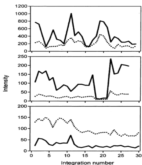
Figure 1. Time dependence of the intensities of the S- (solid) and P- (dotted) polarized Raman scattering from three different SERS-active aggregates. The scattering is excited by 514.5 nm, S-polarized light; all the Stokes (and anti-Stokes) shifted light contributes to the signal. The integrations are 1 s long and taken continuously at 2 s intervals.
