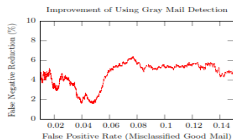
Figure 2: The improvement of using the two-filter architecture compared to the regular spam filter in reducing false negative messages (i.e., unfiltered spam)
