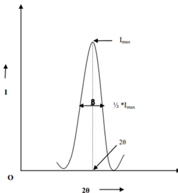
Figure 5: Evaluation of grain size utilising Debye-Scherrer's X-ray peak
