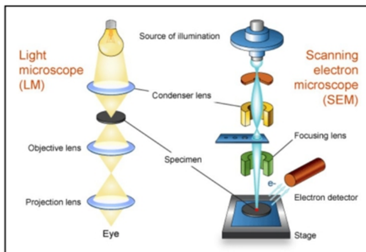
Figure 6: Comparison of Scanning Electron Microscopes with Optical Microscopes
