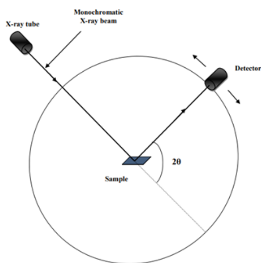
Figure 4: Illustration of an X-ray diffractometer
