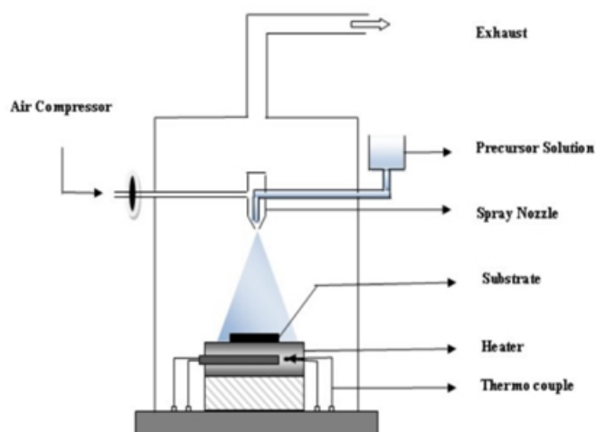
Figure 1: Chemical Spray Pyrolysis Unit Diagram
