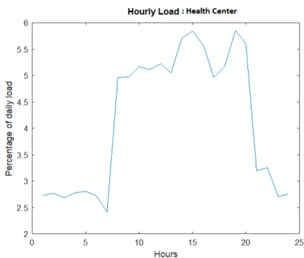
Figure 6: Load Profile for the Health Centre
