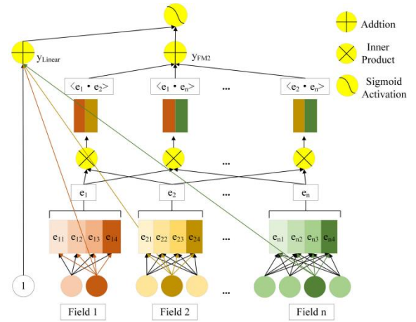
Figure 6 Overall structure diagram of FM
