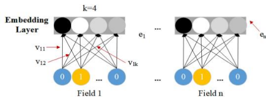
Figure 5 Embedding layer of FM
