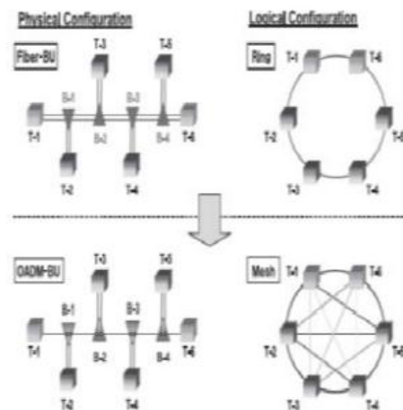
Fig.5. Optical Network Configurations [8]
