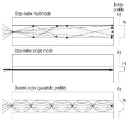
Fig.2. Optical Fiber Modes [6]
