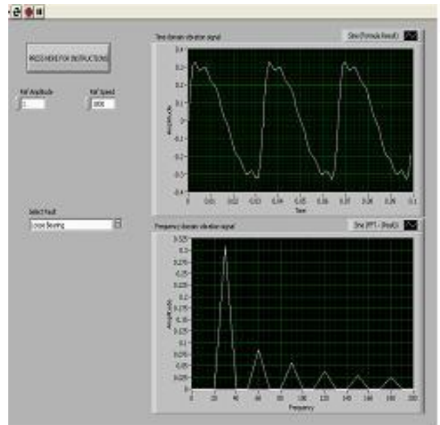
Fig.7 Loose Bearing
