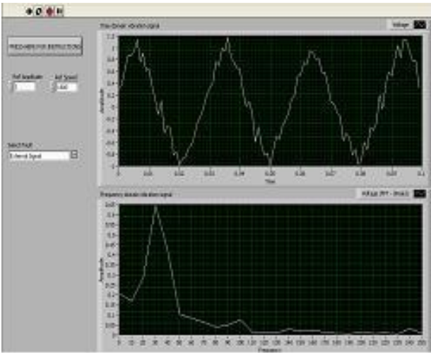
Fig 12 Highest vibration Level (Magnet attached at hinge)
