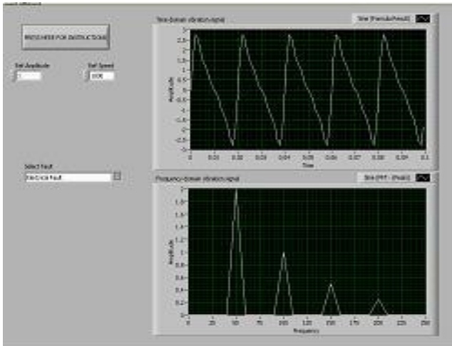
Fig.5 Electrical Fault
