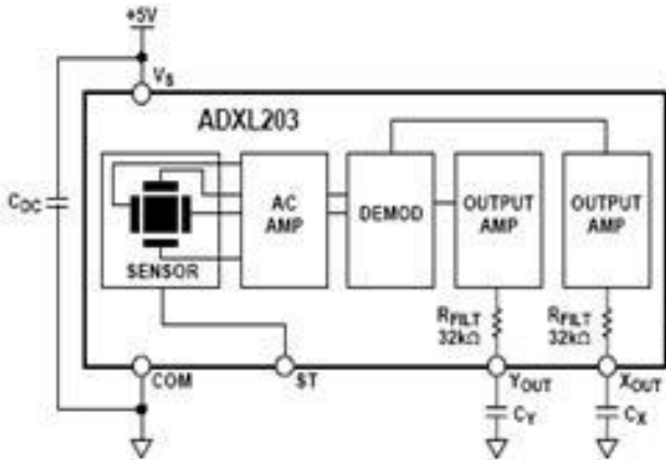
Fig. 8 Block diagram of ADXL 203[11]
