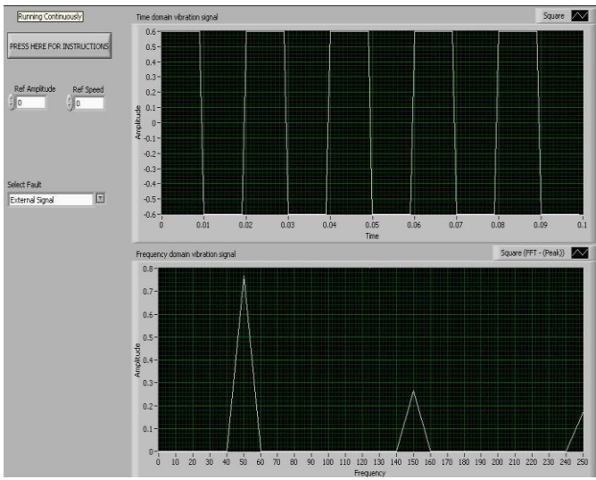
Fig.1 Rectangular waveform interfaced with PCI-6221
