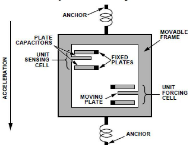
Fig. 9 Internal Arrangement in IC Accelerometer
