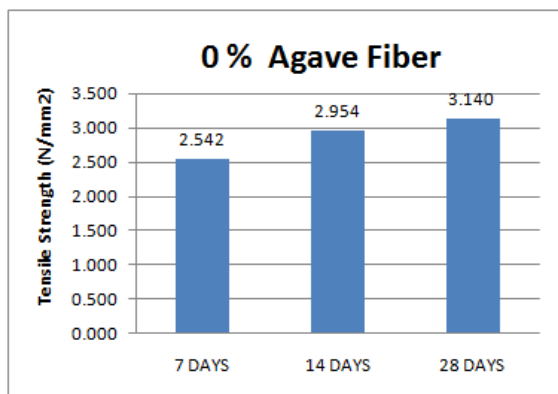
Tensile Strength (0%, 1%,2%, 3% ,4%)
