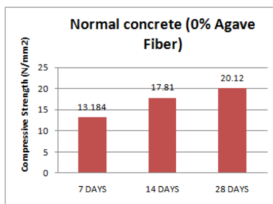
Compressive strength (0%, 1%,2%, 3% ,4%, 5%)
