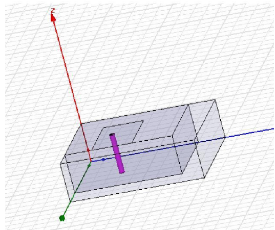
Fig 5 Co-axial Probe Feed
