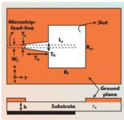
Fig 4 Geometry of Printed Slot Antenna
