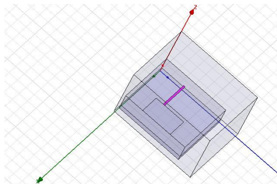
Fig 8 Proximity Coupling Feed
