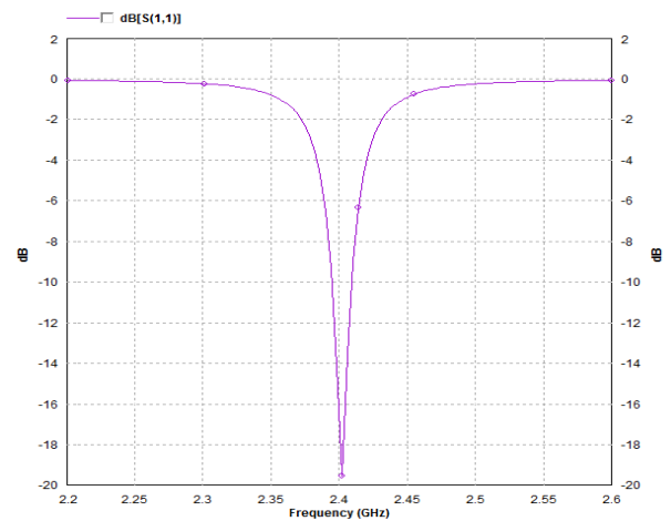
Figure7. Return loss curve for Quarterwave Line Feed.
