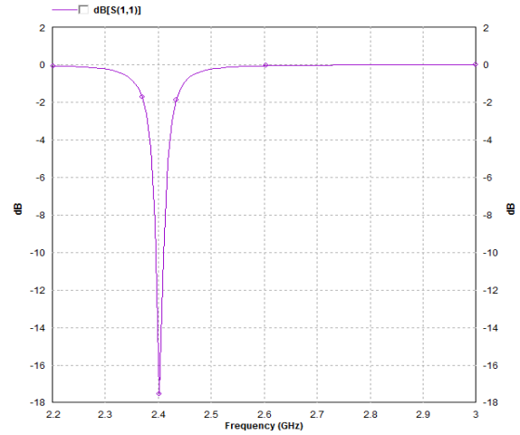
Figure 5. Return loss curve for Strip Feed.
