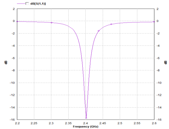
Figure 6. Return loss curve for Inset Line Feed.
