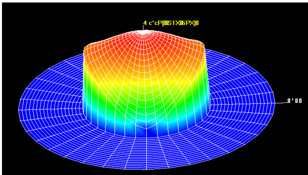
Figure 9. 3D View of Current Distribution for Inset Line Feed.
