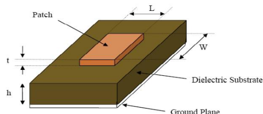
Figure1. Basic Microstrip Patch.
