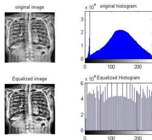
Fig 2: Histogram Equalization
