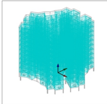
Figure 5: Analytical model of G+10 residential building
