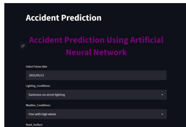
Figure 14: Web page
