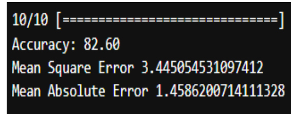
Figure 16: Model accuracy
