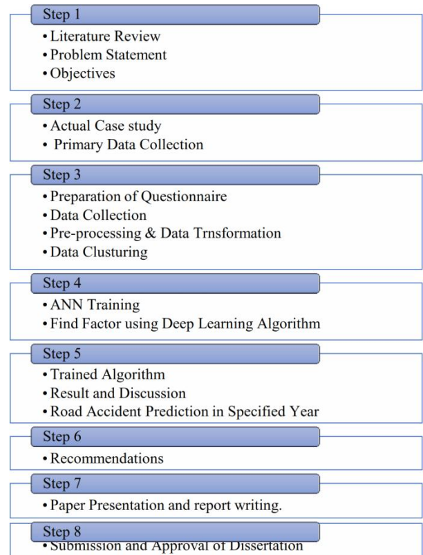
Figure 5: Methodology Flow
