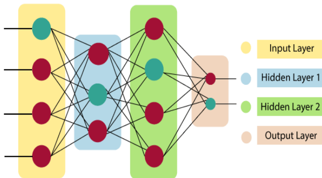
Figure 3: ANN architecture
