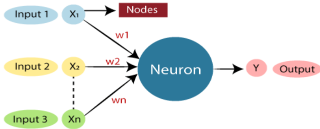
Figure 2: ANN network
