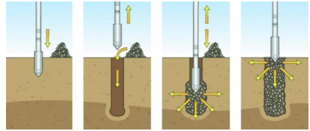
Fig:1.4: Step by Step Stone Column
