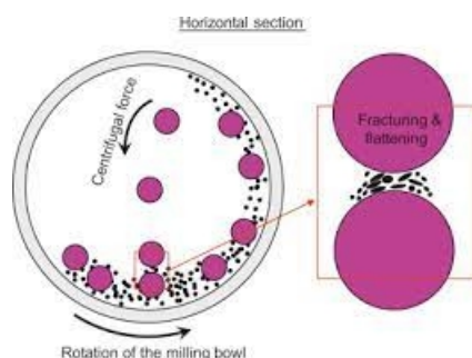
Figure 3: Ball mill
