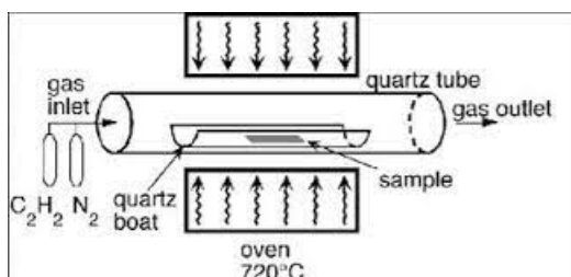
Figure 5: Chemical vapour deposition
