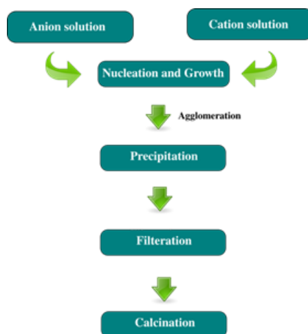
Figure 8: Co-precipitation method
