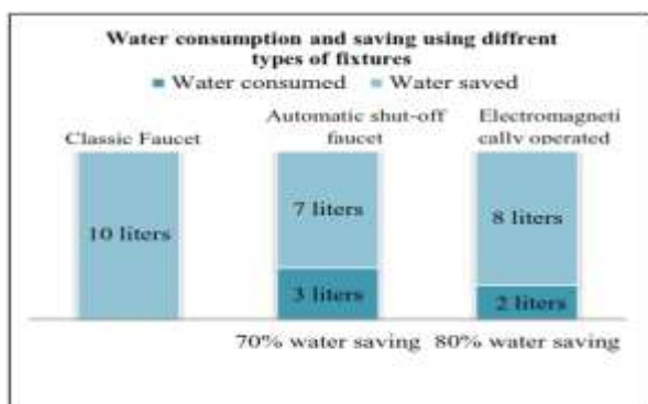
Chart 1. Water consumption and saving using different types of fixtures
